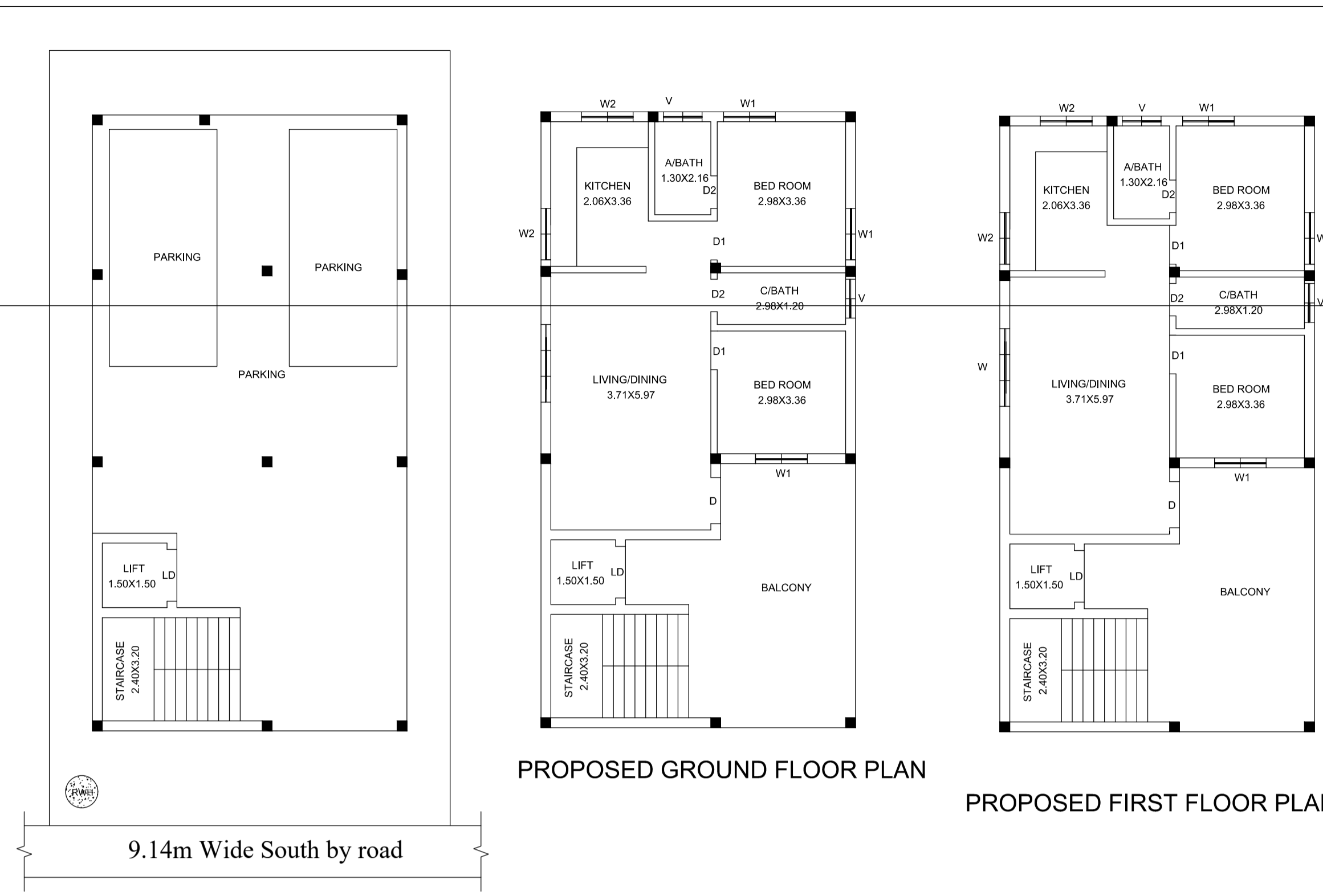
PROPOSED SITE FLOOR PLAN
